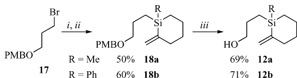
Scheme 11. Preparation of (3-hydroxypropyl)silanes 12 from the bromopropanol derivative 17 . Reagents and conditions: i ) Mg, THF, 60 °C; ii ) 8a or 8b (0.9 equiv.), THF, 20 °C, 1.4 h; iii ) DDQ (1.3 equiv.), DCM/H 2 O, 20 °C, 0.5 h.
