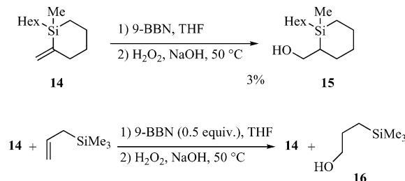
Scheme 9. Hydroboration of vinylsilane 14 and allyltrimethylsilane.
