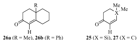
Figure 4. Selected cycloalkenones for NMR comparison.
