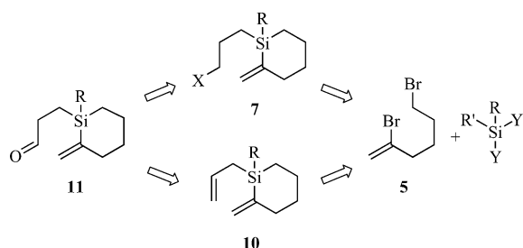
Scheme 3. Retrosynthesis of 2-methylidene-1-silacyclohexanes 11 .
