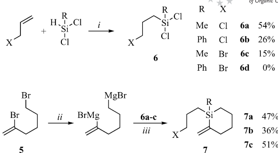
Scheme 4. Preparation of 3-halopropylsilanes 7 . Reagents and conditions: i) for 6a and 6c , [H 2 PtCl 6 ], cyclohexane, reflux, 14 h; for 6b and 6d , [H 2 PtCl 6 ], without solvent; ii) THF, addition of 5 at 10 °C, then 3 h at 20 °C; iii) Grignard reagent (1 equiv.), THF, 65 °C, 1.4 h.
