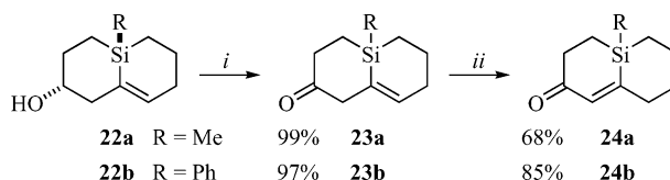
Scheme 14. Preparation of silabicyclodec-5-en-4-ones 24 . Reagents and conditions: i) \text{CrO}_3/\text{H}_2\text{SO}_4 , acetone, 20 °C, 10 min; ii) KOH (cat.), MeOH, 50–60 °C, 50 min, then neutralization with acetic acid.
