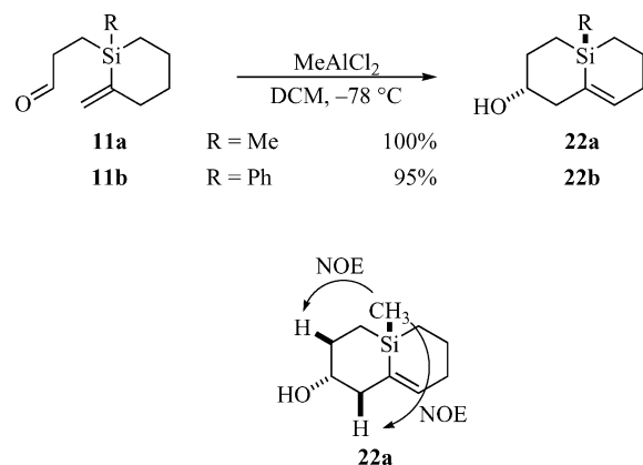
Scheme 13. Preparation of silabicyclodec-6-en-4-ols 22 by the ene reaction and NOE effects.
