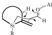
Figure 3. Dreiding model of the ene reaction with aldehydes 11 .
