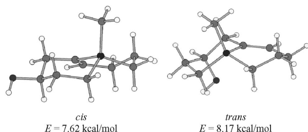
Figure 2. MM + -minimized geometries of the cis and trans isomers 22a .
