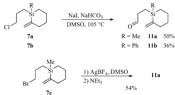
Scheme 5. Preparation of 3-oxopropylsilanes 11 from halopropylsilanes.
