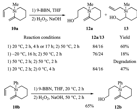
Scheme 8. Formation of (3-hydroxypropyl)silanes 12 from the allylsilanes 10 .
