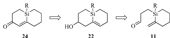
Scheme 2. Retrosynthesis of 1-silabicyclo[4.4.0]dec-5-en-4-ones 24 .
