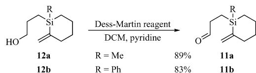
Scheme 10. Preparation of 3-oxopropylsilanes 11 from alcohols 12 .
